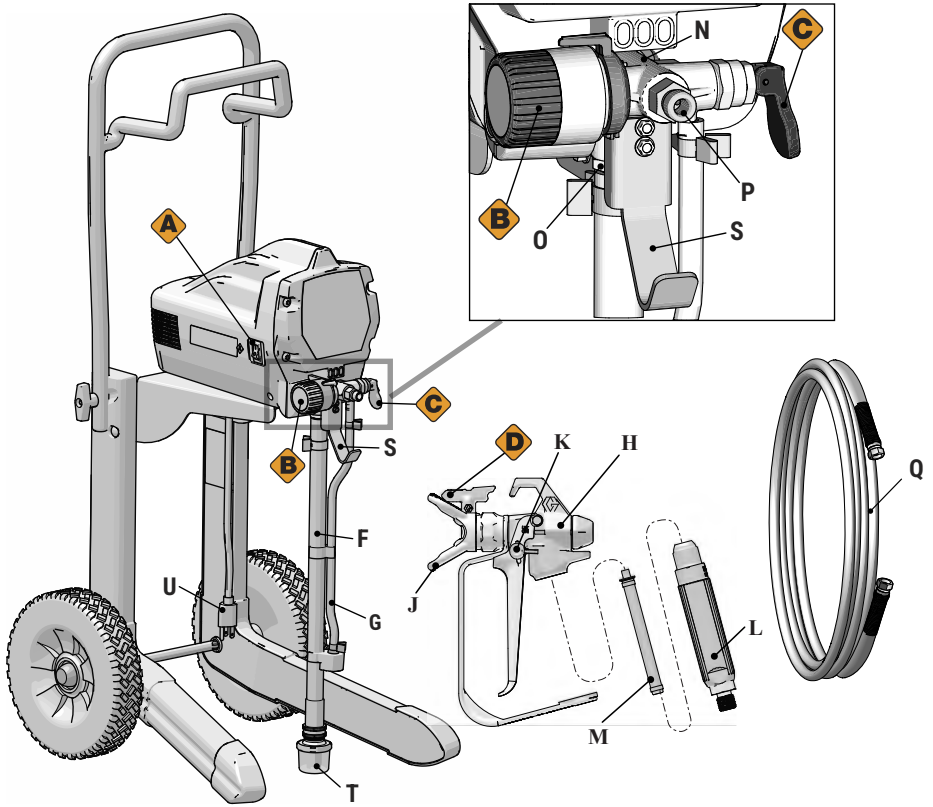
Figure 7-3: X7 Cart Diagram
